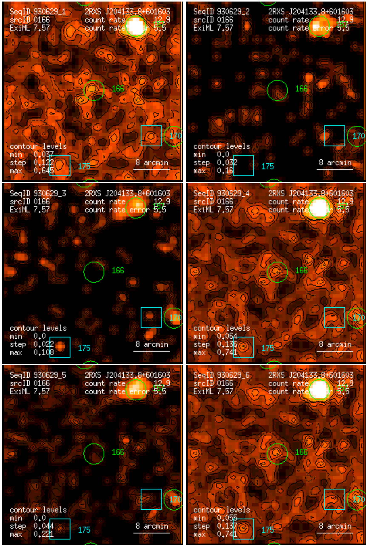
Figure 166: RASS 930629: detection 0166: band rate images, Gaussian filter: (1) PSPC channels 11 – 41, (2) 52 – 90, (3) 91 – 201, (4) 11 – 235, (5) 52 – 201, (6) 11 – 201. Broad band rates in counts/ks. Band rate contour levels in counts/ks/arcmin 2 .
