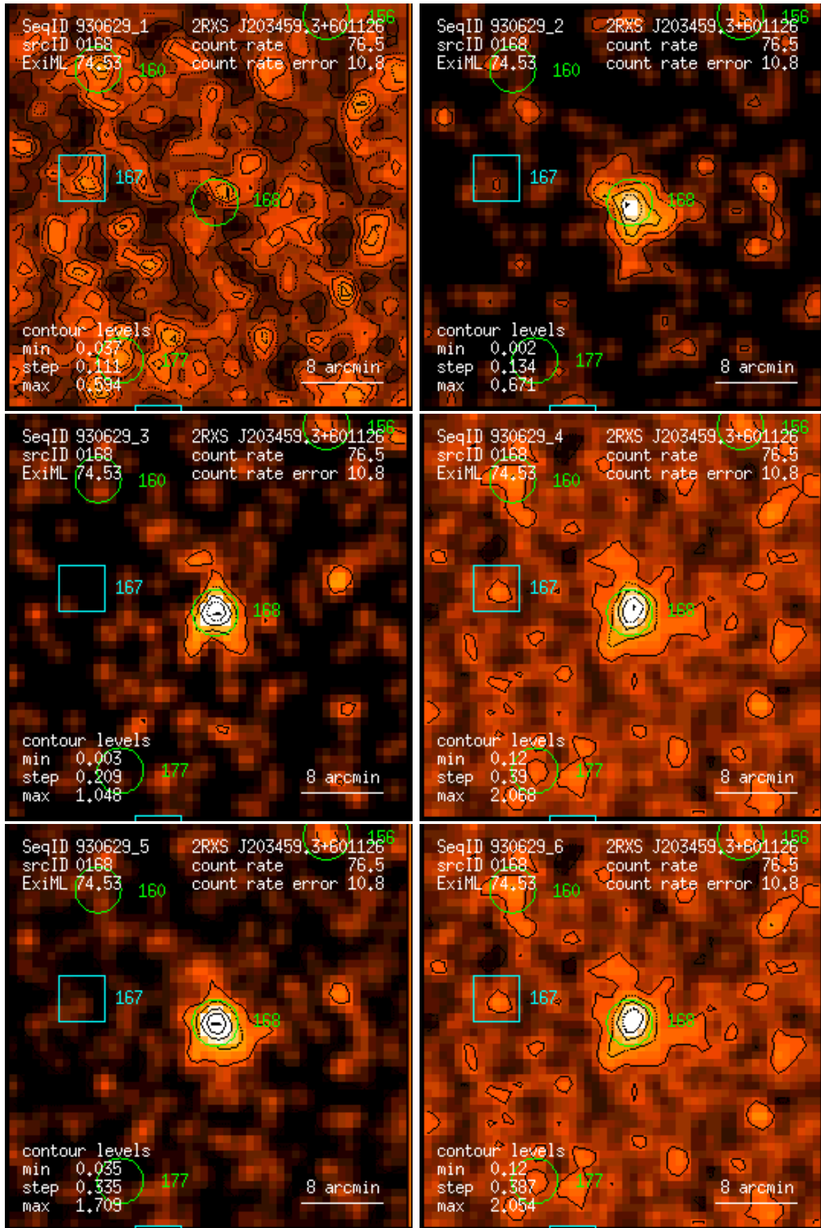
Figure 168: RASS 930629: detection 0168: band rate images, Gaussian filter: (1) PSPC channels 11 – 41, (2) 52 – 90, (3) 91 – 201, (4) 11 – 235, (5) 52 – 201, (6) 11 – 201. Broad band rates in counts/ks. Band rate contour levels in counts/ks/arcmin 2 .
