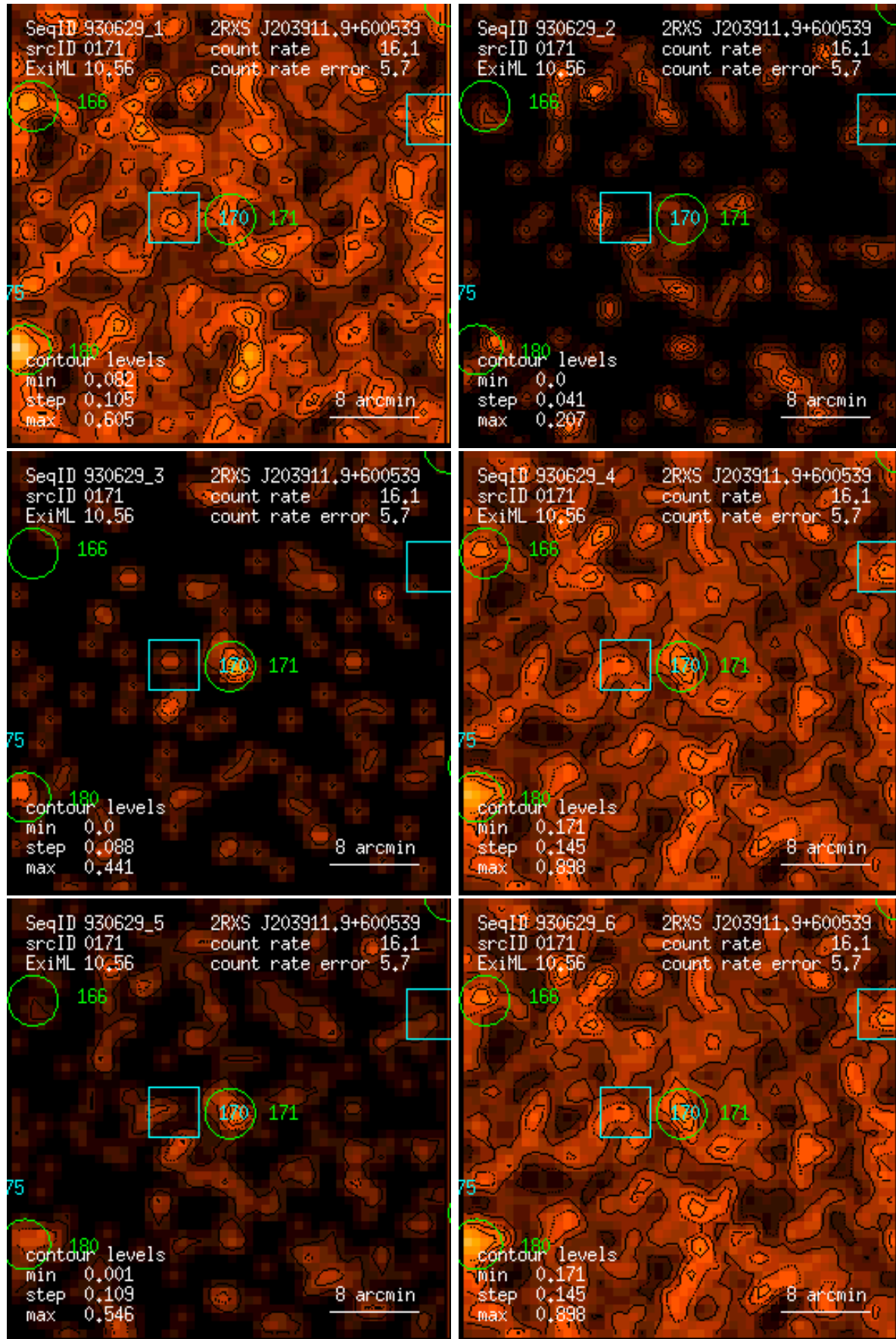
Figure 171: RASS 930629: detection 0171: band rate images, Gaussian filter: (1) PSPC channels 11 – 41, (2) 52 – 90, (3) 91 – 201, (4) 11 – 235, (5) 52 – 201, (6) 11 – 201. Broad band rates in counts/ks. Band rate contour levels in counts/ks/arcmin 2 .
