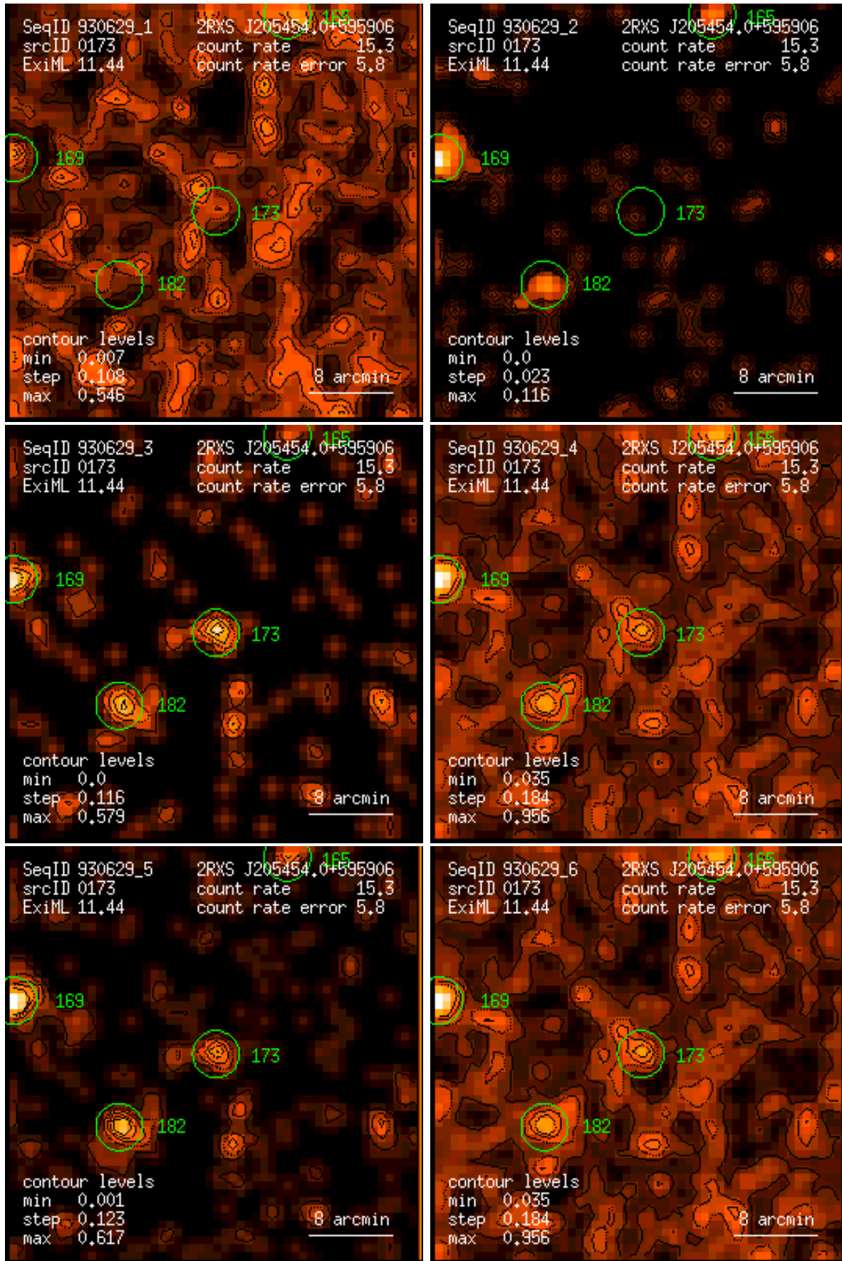
Figure 173: RASS 930629: detection 0173: band rate images, Gaussian filter: (1) PSPC channels 11 – 41, (2) 52 – 90, (3) 91 – 201, (4) 11 – 235, (5) 52 – 201, (6) 11 – 201. Broad band rates in counts/ks. Band rate contour levels in counts/ks/arcmin 2 .
