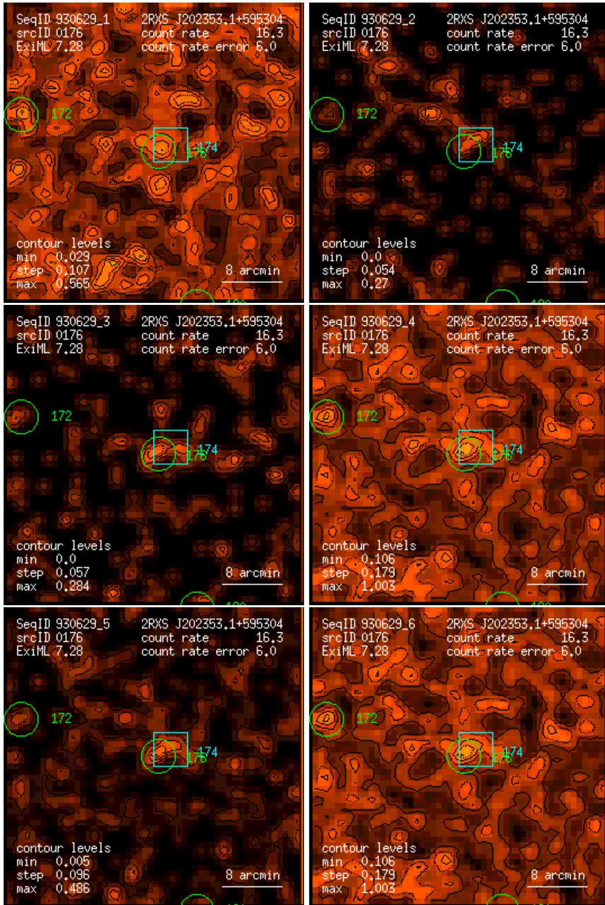
Figure 176: RASS 930629: detection 0176: band rate images, Gaussian filter: (1) PSPC channels 11 – 41, (2) 52 – 90, (3) 91 – 201, (4) 11 – 235, (5) 52 – 201, (6) 11 – 201. Broad band rates in counts/ks. Band rate contour levels in counts/ks/arcmin 2 .
