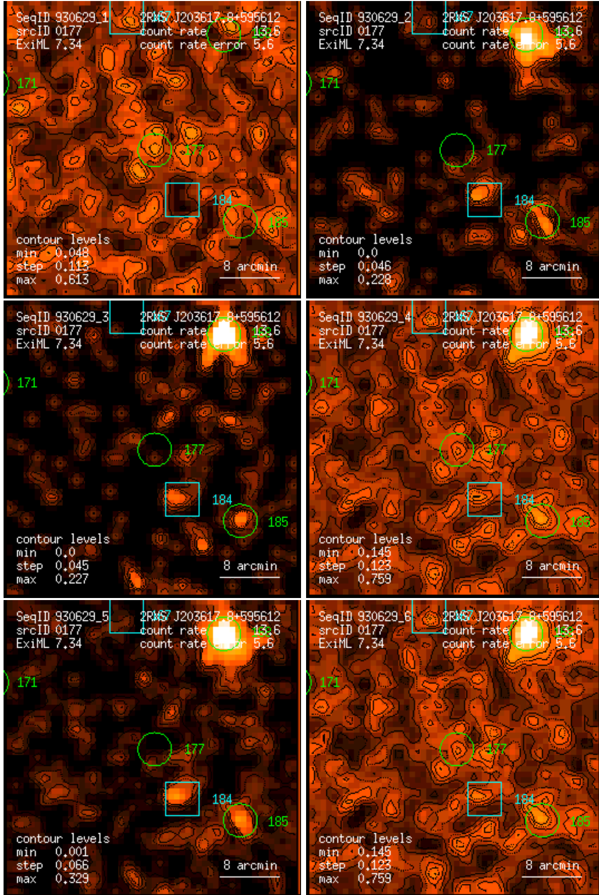
Figure 177: RASS 930629: detection 0177: band rate images, Gaussian filter: (1) PSPC channels 11 – 41, (2) 52 – 90, (3) 91 – 201, (4) 11 – 235, (5) 52 – 201, (6) 11 – 201. Broad band rates in counts/ks. Band rate contour levels in counts/ks/arcmin 2 .
