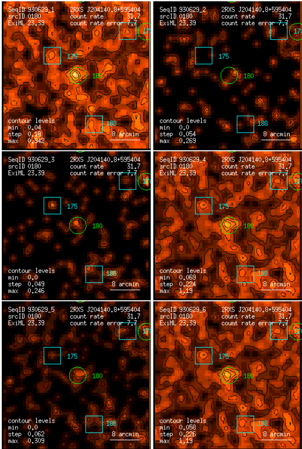
Figure 180: RASS 930629: detection 0180: band rate images, Gaussian filter: (1) PSPC channels 11 – 41, (2) 52 – 90, (3) 91 – 201, (4) 11 – 235, (5) 52 – 201, (6) 11 – 201. Broad band rates in counts/ks. Band rate contour levels in counts/ks/arcmin 2 .
