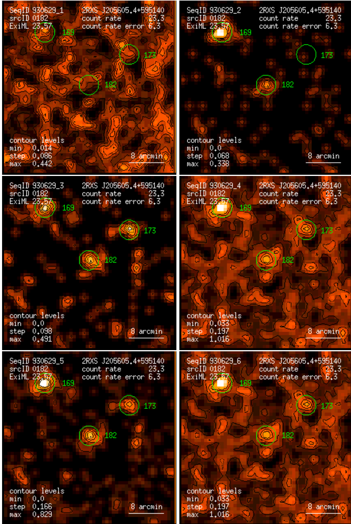
Figure 182: RASS 930629: detection 0182: band rate images, Gaussian filter: (1) PSPC channels 11 – 41, (2) 52 – 90, (3) 91 – 201, (4) 11 – 235, (5) 52 – 201, (6) 11 – 201. Broad band rates in counts/ks. Band rate contour levels in counts/ks/arcmin 2 .
