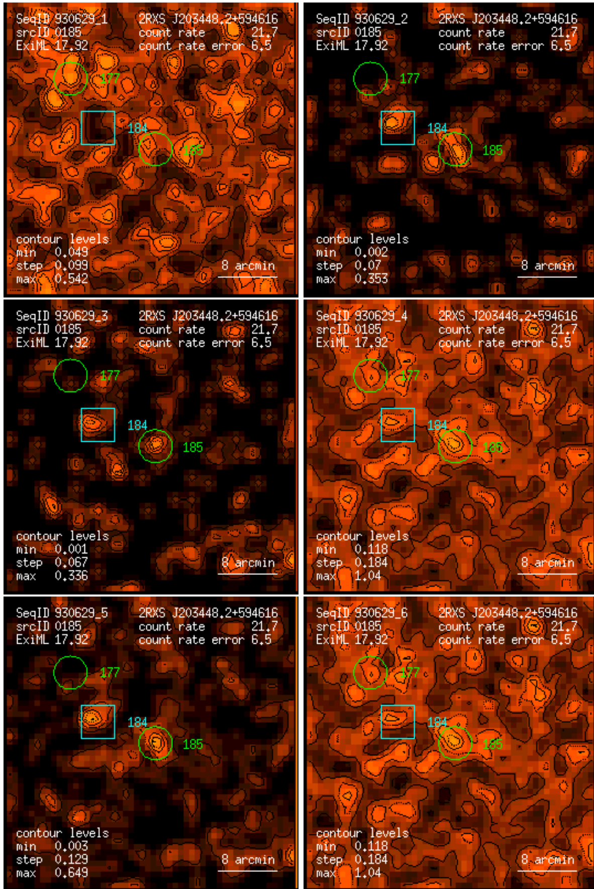
Figure 185: RASS 930629: detection 0185: band rate images, Gaussian filter: (1) PSPC channels 11 – 41, (2) 52 – 90, (3) 91 – 201, (4) 11 – 235, (5) 52 – 201, (6) 11 – 201. Broad band rates in counts/ks. Band rate contour levels in counts/ks/arcmin 2 .
