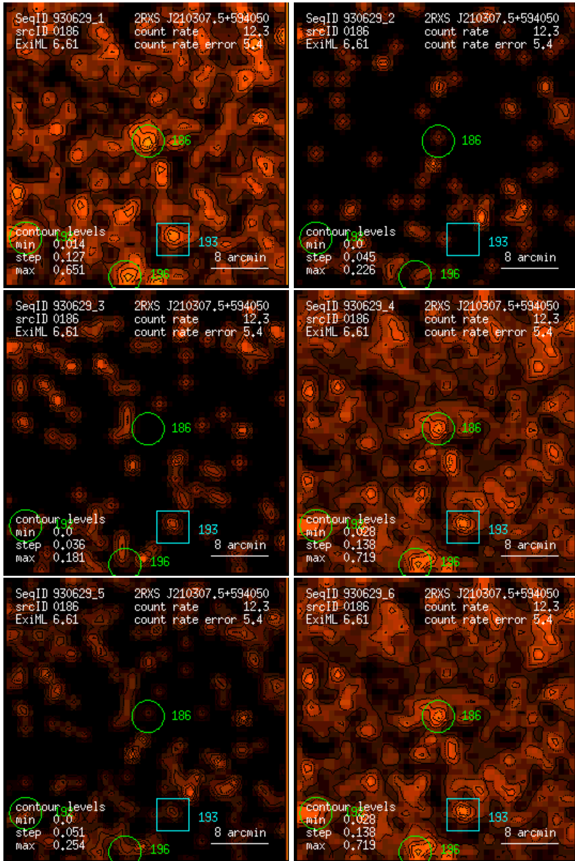
Figure 186: RASS 930629: detection 0186: band rate images, Gaussian filter: (1) PSPC channels 11 – 41, (2) 52 – 90, (3) 91 – 201, (4) 11 – 235, (5) 52 – 201, (6) 11 – 201. Broad band rates in counts/ks. Band rate contour levels in counts/ks/arcmin 2 .
