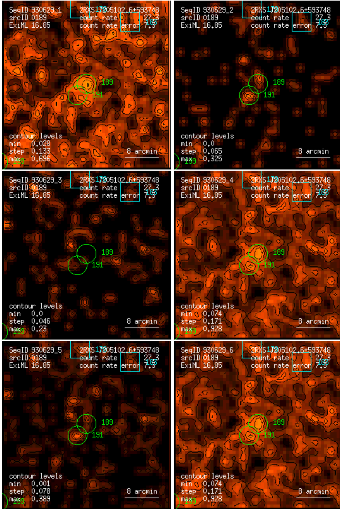
Figure 189: RASS 930629: detection 0189: band rate images, Gaussian filter: (1) PSPC channels 11 – 41, (2) 52 – 90, (3) 91 – 201, (4) 11 – 235, (5) 52 – 201, (6) 11 – 201. Broad band rates in counts/ks. Band rate contour levels in counts/ks/arcmin 2 .
