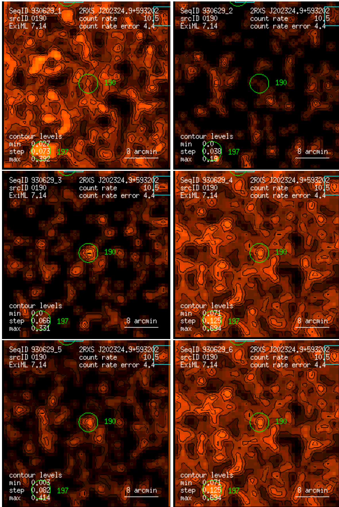
Figure 190: RASS 930629: detection 0190: band rate images, Gaussian filter: (1) PSPC channels 11 – 41, (2) 52 – 90, (3) 91 – 201, (4) 11 – 235, (5) 52 – 201, (6) 11 – 201. Broad band rates in counts/ks. Band rate contour levels in counts/ks/arcmin 2 .
