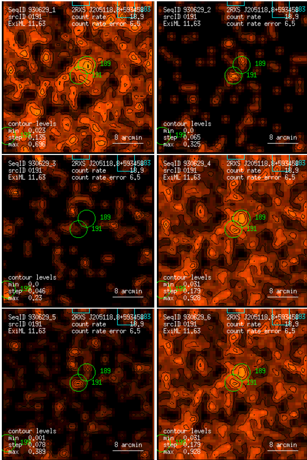
Figure 191: RASS 930629: detection 0191: band rate images, Gaussian filter: (1) PSPC channels 11 – 41, (2) 52 – 90, (3) 91 – 201, (4) 11 – 235, (5) 52 – 201, (6) 11 – 201. Broad band rates in counts/ks. Band rate contour levels in counts/ks/arcmin 2 .
