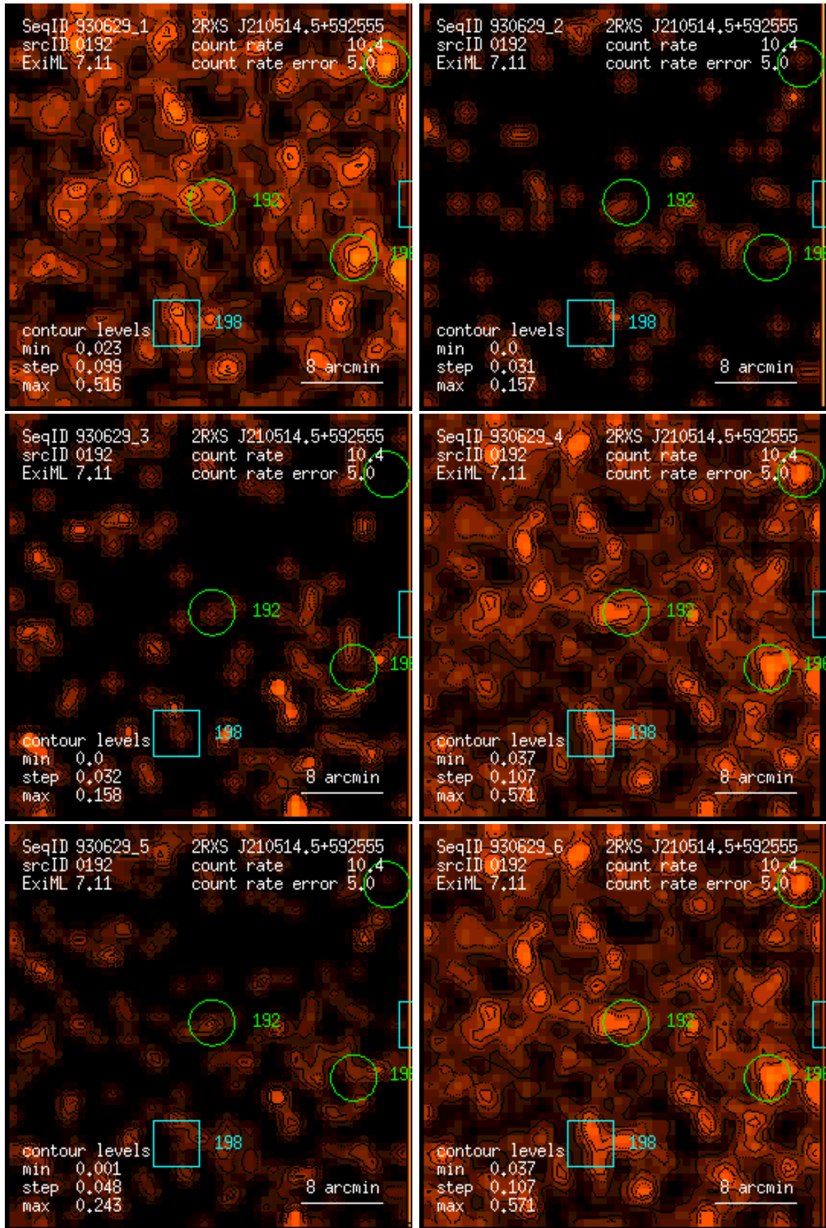
Figure 192: RASS 930629: detection 0192: band rate images, Gaussian filter: (1) PSPC channels 11 – 41, (2) 52 – 90, (3) 91 – 201, (4) 11 – 235, (5) 52 – 201, (6) 11 – 201. Broad band rates in counts/ks. Band rate contour levels in counts/ks/arcmin 2 .
