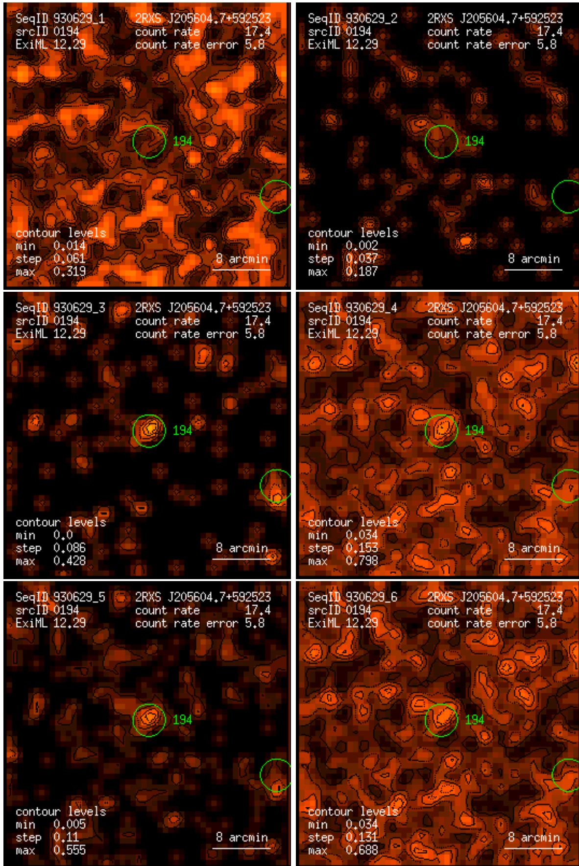
Figure 194: RASS 930629: detection 0194: band rate images, Gaussian filter: (1) PSPC channels 11 – 41, (2) 52 – 90, (3) 91 – 201, (4) 11 – 235, (5) 52 – 201, (6) 11 – 201. Broad band rates in counts/ks. Band rate contour levels in counts/ks/arcmin 2 .
