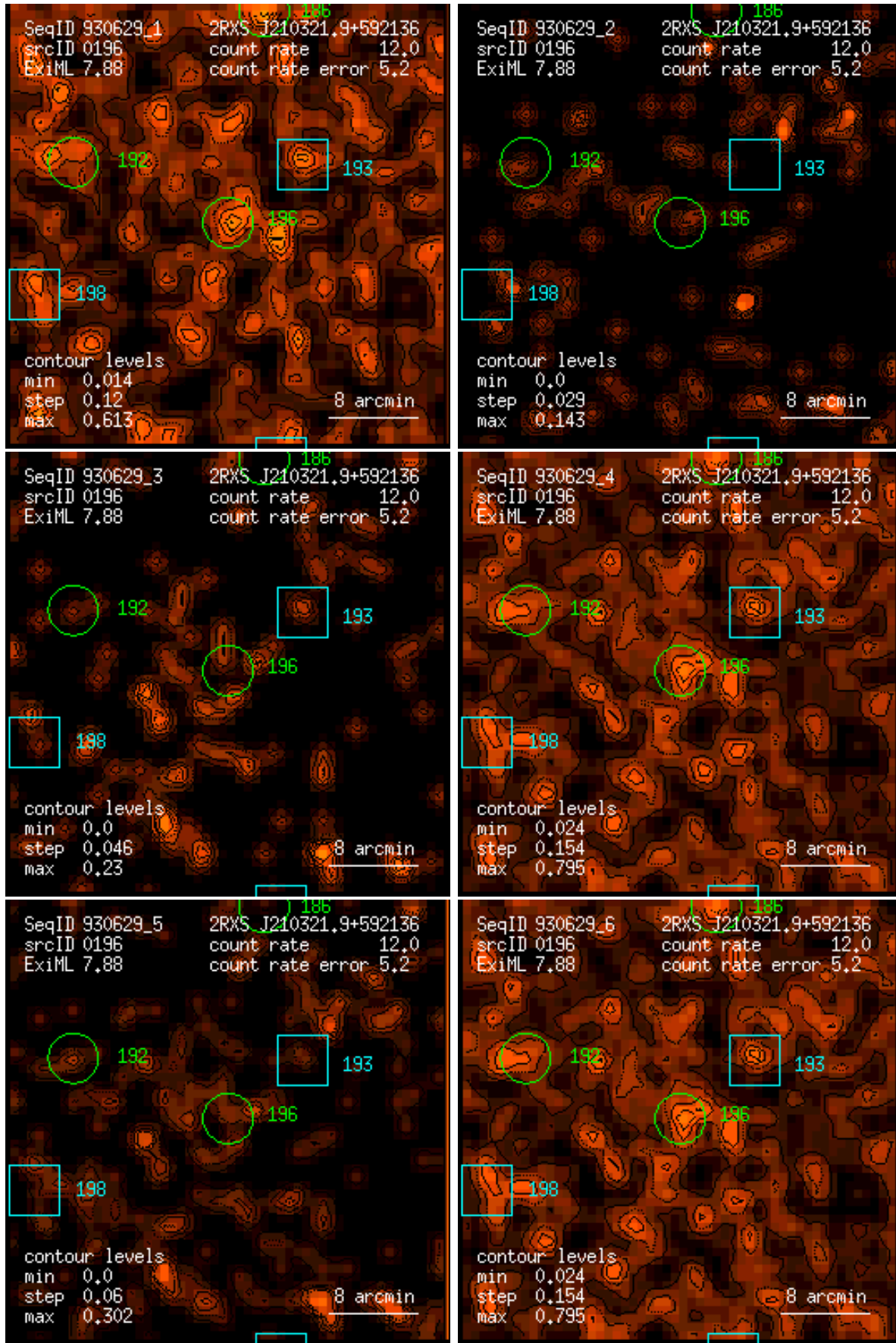
Figure 196: RASS 930629: detection 0196: band rate images, Gaussian filter: (1) PSPC channels 11 – 41, (2) 52 – 90, (3) 91 – 201, (4) 11 – 235, (5) 52 – 201, (6) 11 – 201. Broad band rates in counts/ks. Band rate contour levels in counts/ks/arcmin 2 .
