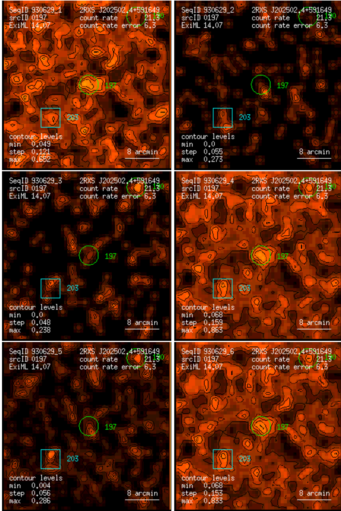
Figure 197: RASS 930629: detection 0197: band rate images, Gaussian filter: (1) PSPC channels 11 – 41, (2) 52 – 90, (3) 91 – 201, (4) 11 – 235, (5) 52 – 201, (6) 11 – 201. Broad band rates in counts/ks. Band rate contour levels in counts/ks/arcmin 2 .
