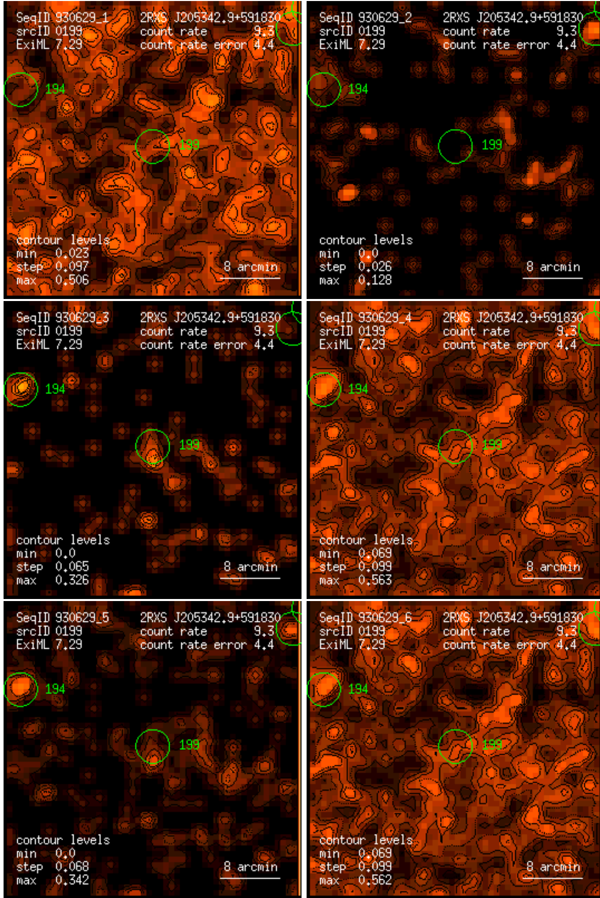
Figure 199: RASS 930629: detection 0199: band rate images, Gaussian filter: (1) PSPC channels 11 – 41, (2) 52 – 90, (3) 91 – 201, (4) 11 – 235, (5) 52 – 201, (6) 11 – 201. Broad band rates in counts/ks. Band rate contour levels in counts/ks/arcmin 2 .
