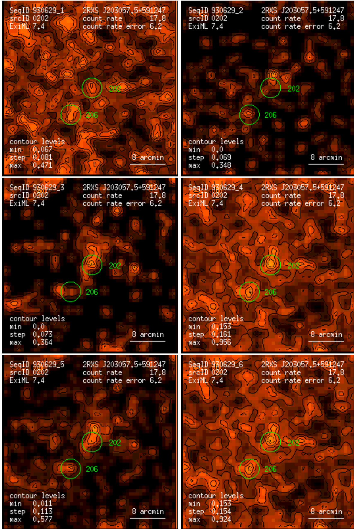
Figure 202: RASS 930629: detection 0202: band rate images, Gaussian filter: (1) PSPC channels 11 – 41, (2) 52 – 90, (3) 91 – 201, (4) 11 – 235, (5) 52 – 201, (6) 11 – 201. Broad band rates in counts/ks. Band rate contour levels in counts/ks/arcmin 2 .
