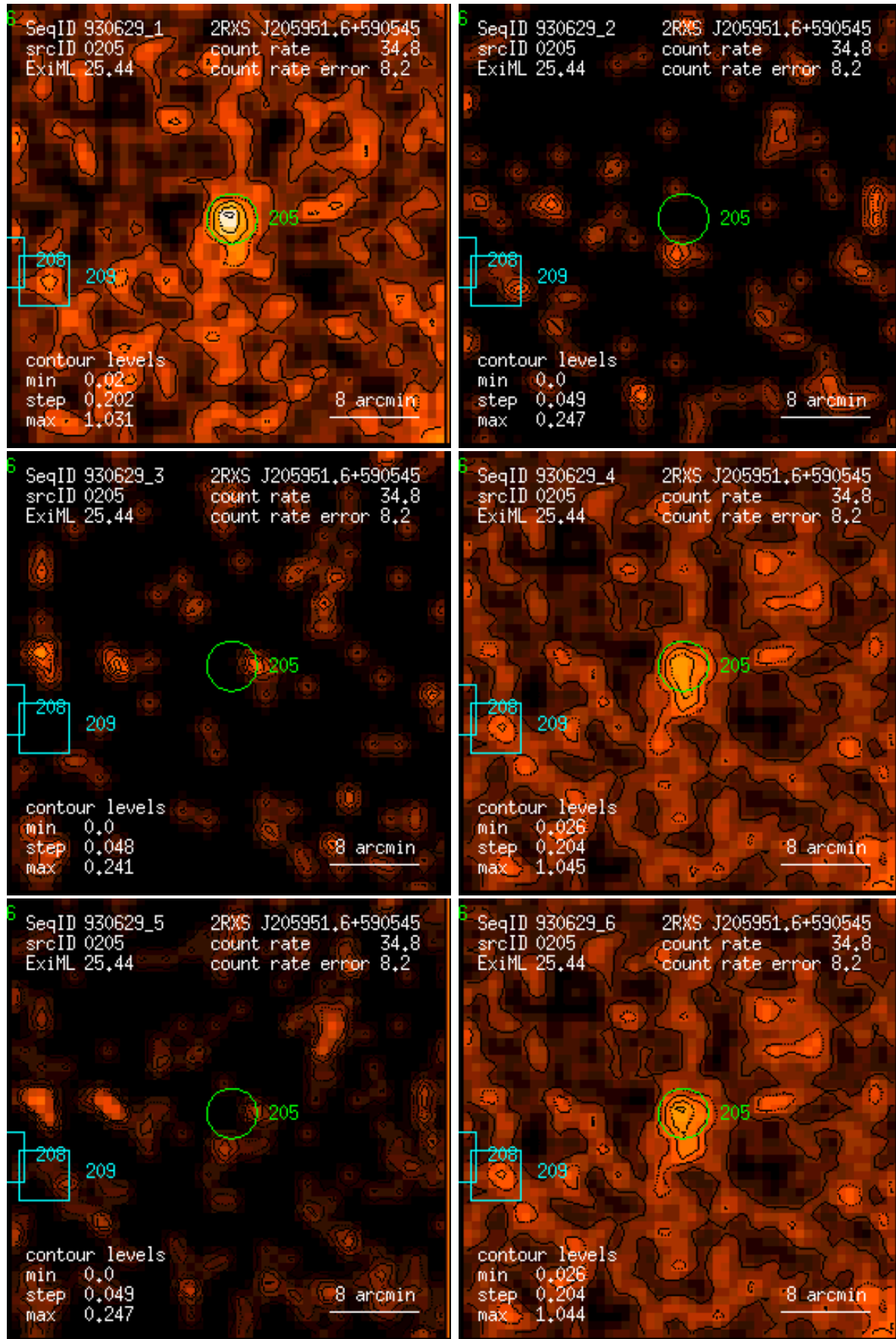
Figure 205: RASS 930629: detection 0205: band rate images, Gaussian filter: (1) PSPC channels 11 – 41, (2) 52 – 90, (3) 91 – 201, (4) 11 – 235, (5) 52 – 201, (6) 11 – 201. Broad band rates in counts/ks. Band rate contour levels in counts/ks/arcmin 2 .
