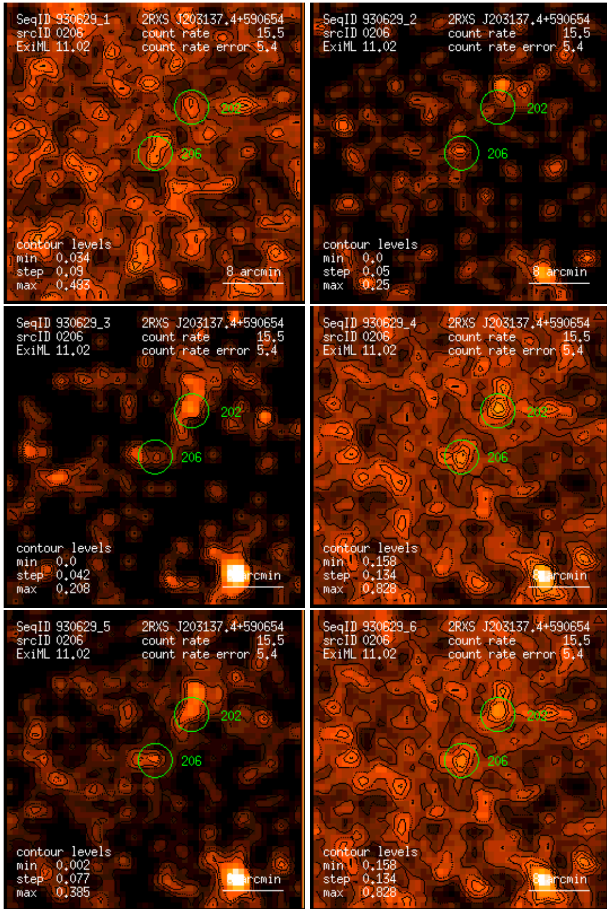
Figure 206: RASS 930629: detection 0206: band rate images, Gaussian filter: (1) PSPC channels 11 – 41, (2) 52 – 90, (3) 91 – 201, (4) 11 – 235, (5) 52 – 201, (6) 11 – 201. Broad band rates in counts/ks. Band rate contour levels in counts/ks/arcmin 2 .
