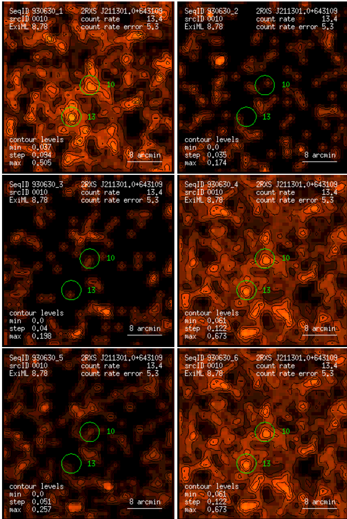
Figure 10: RASS 930630: detection 0010: band rate images, Gaussian filter: (1) PSPC channels 11 – 41, (2) 52 – 90, (3) 91 – 201, (4) 11 – 235, (5) 52 – 201, (6) 11 – 201. Broad band rates in counts/ks. Band rate contour levels in counts/ks/arcmin 2 .
