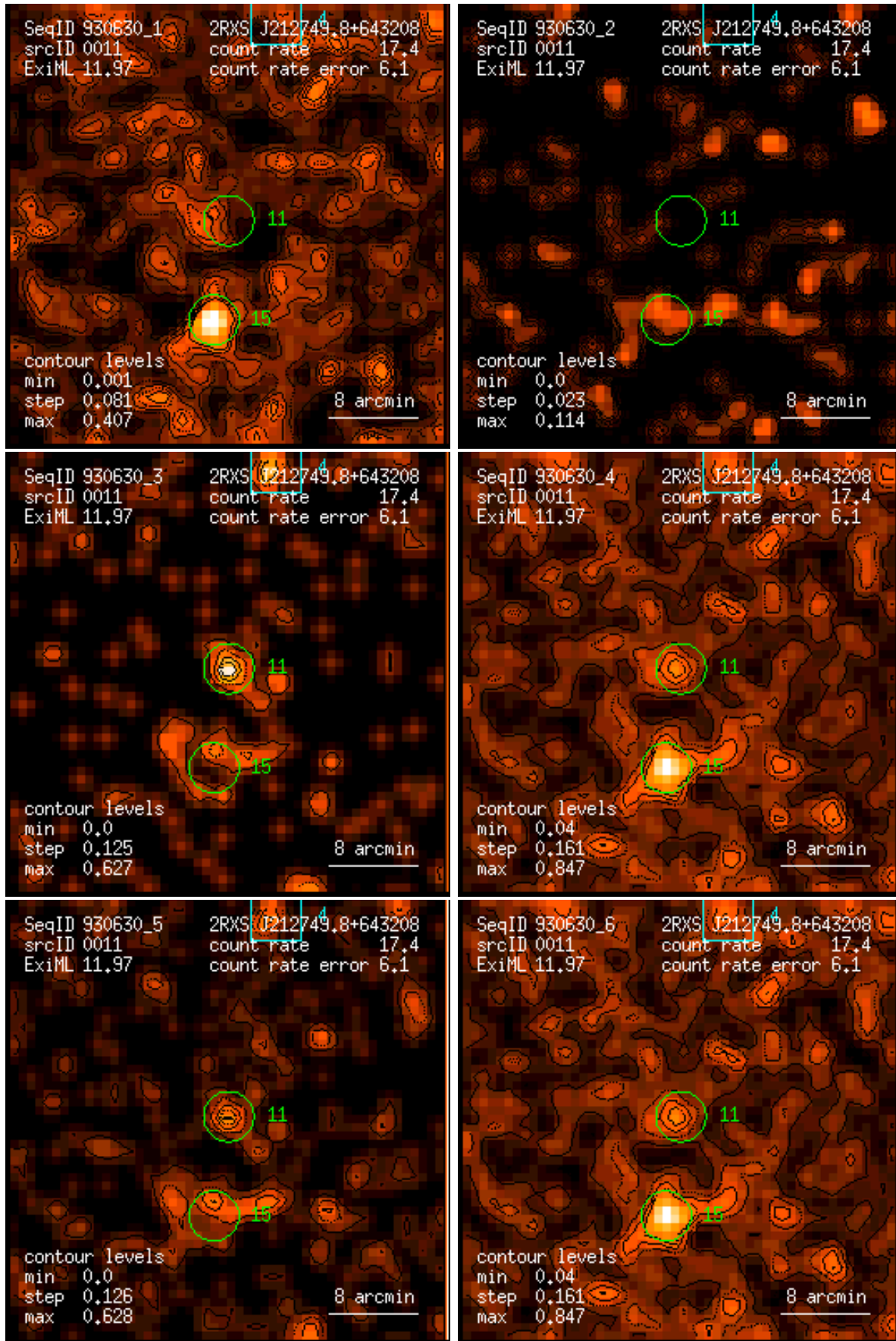
Figure 11: RASS 930630: detection 0011: band rate images, Gaussian filter: (1) PSPC channels 11 – 41, (2) 52 – 90, (3) 91 – 201, (4) 11 – 235, (5) 52 – 201, (6) 11 – 201. Broad band rates in counts/ks. Band rate contour levels in counts/ks/arcmin 2 .
