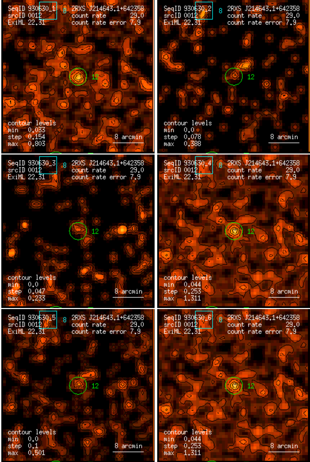
Figure 12: RASS 930630: detection 0012: band rate images, Gaussian filter: (1) PSPC channels 11 – 41, (2) 52 – 90, (3) 91 – 201, (4) 11 – 235, (5) 52 – 201, (6) 11 – 201. Broad band rates in counts/ks. Band rate contour levels in counts/ks/arcmin 2 .
