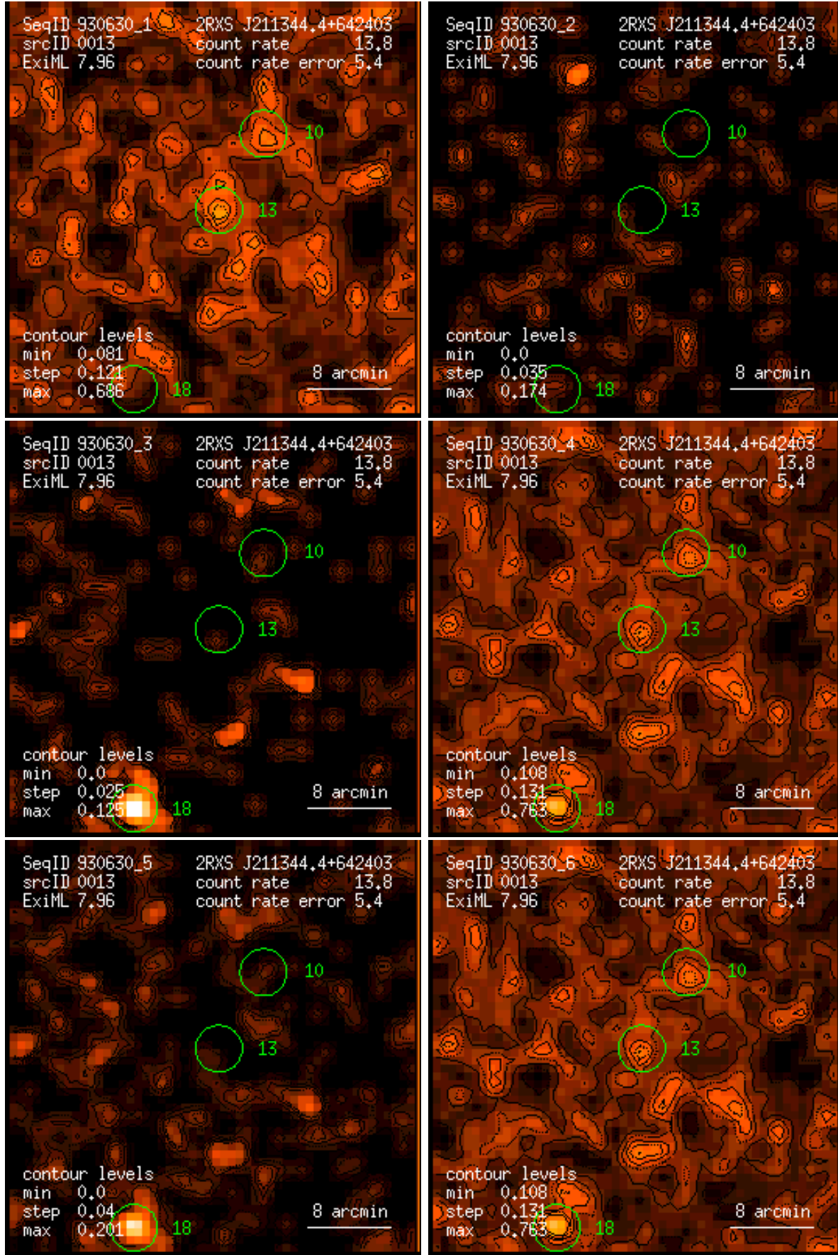
Figure 13: RASS 930630: detection 0013: band rate images, Gaussian filter: (1) PSPC channels 11 – 41, (2) 52 – 90, (3) 91 – 201, (4) 11 – 235, (5) 52 – 201, (6) 11 – 201. Broad band rates in counts/ks. Band rate contour levels in counts/ks/arcmin 2 .
