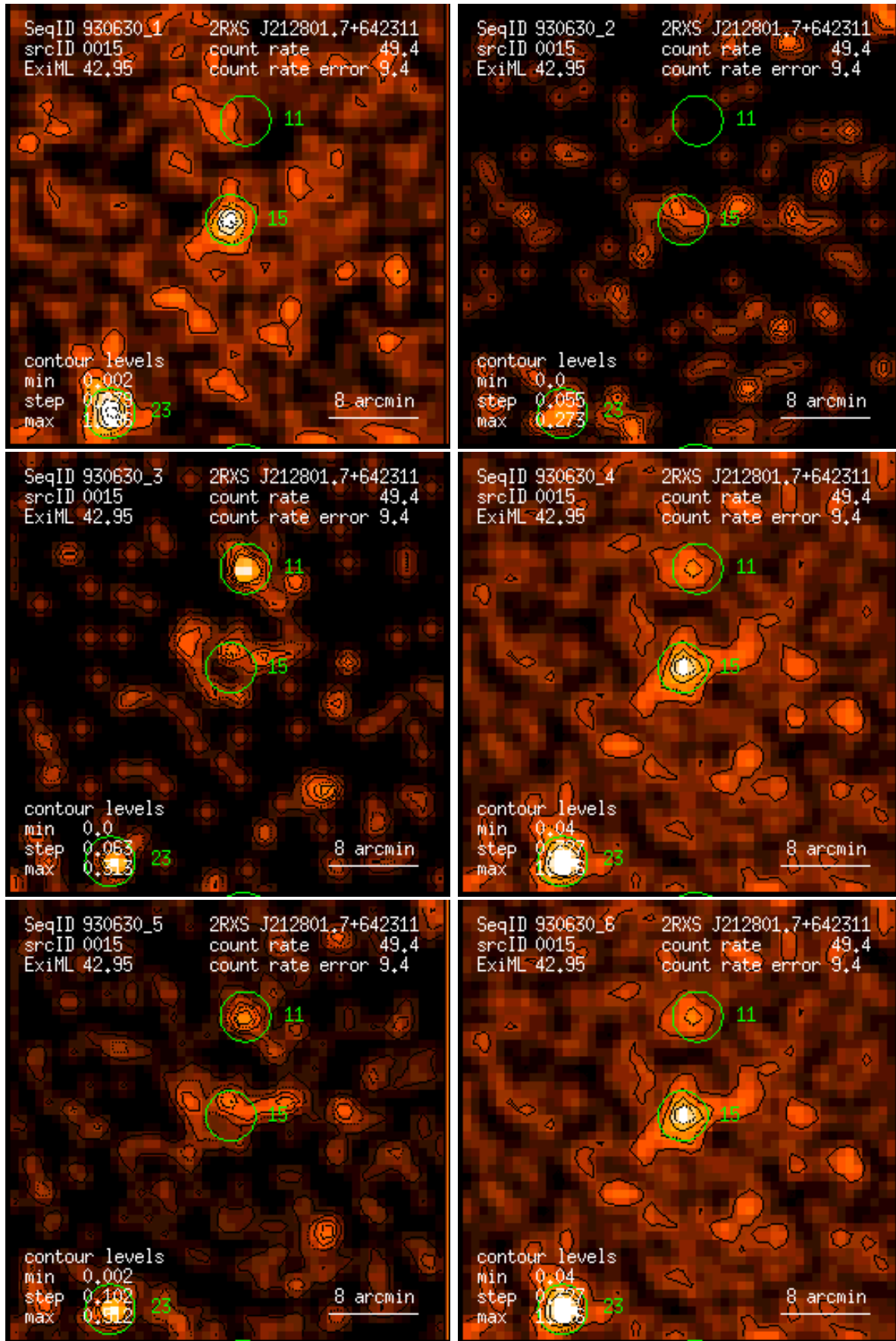
Figure 15: RASS 930630: detection 0015: band rate images, Gaussian filter: (1) PSPC channels 11 – 41, (2) 52 – 90, (3) 91 – 201, (4) 11 – 235, (5) 52 – 201, (6) 11 – 201. Broad band rates in counts/ks. Band rate contour levels in counts/ks/arcmin 2 .
