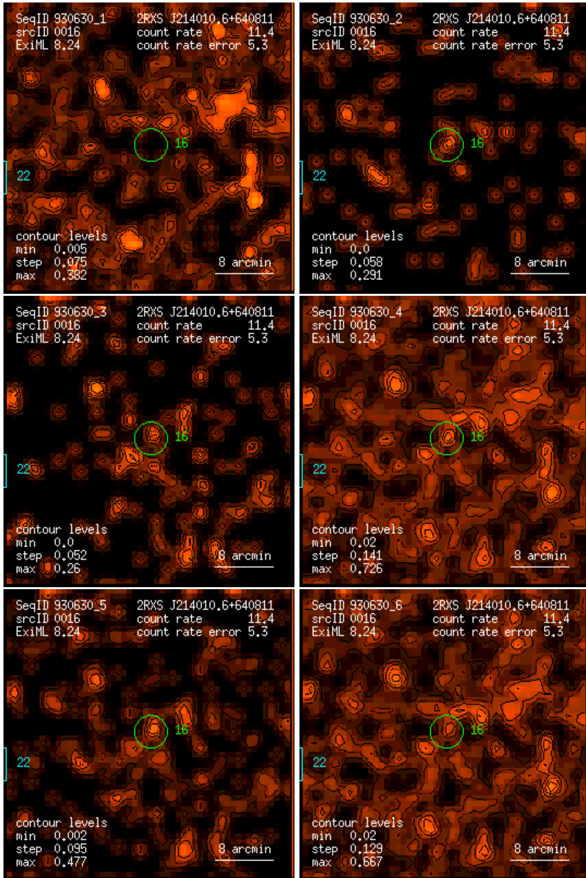
Figure 16: RASS 930630: detection 0016: band rate images, Gaussian filter: (1) PSPC channels 11 – 41, (2) 52 – 90, (3) 91 – 201, (4) 11 – 235, (5) 52 – 201, (6) 11 – 201. Broad band rates in counts/ks. Band rate contour levels in counts/ks/arcmin 2 .
