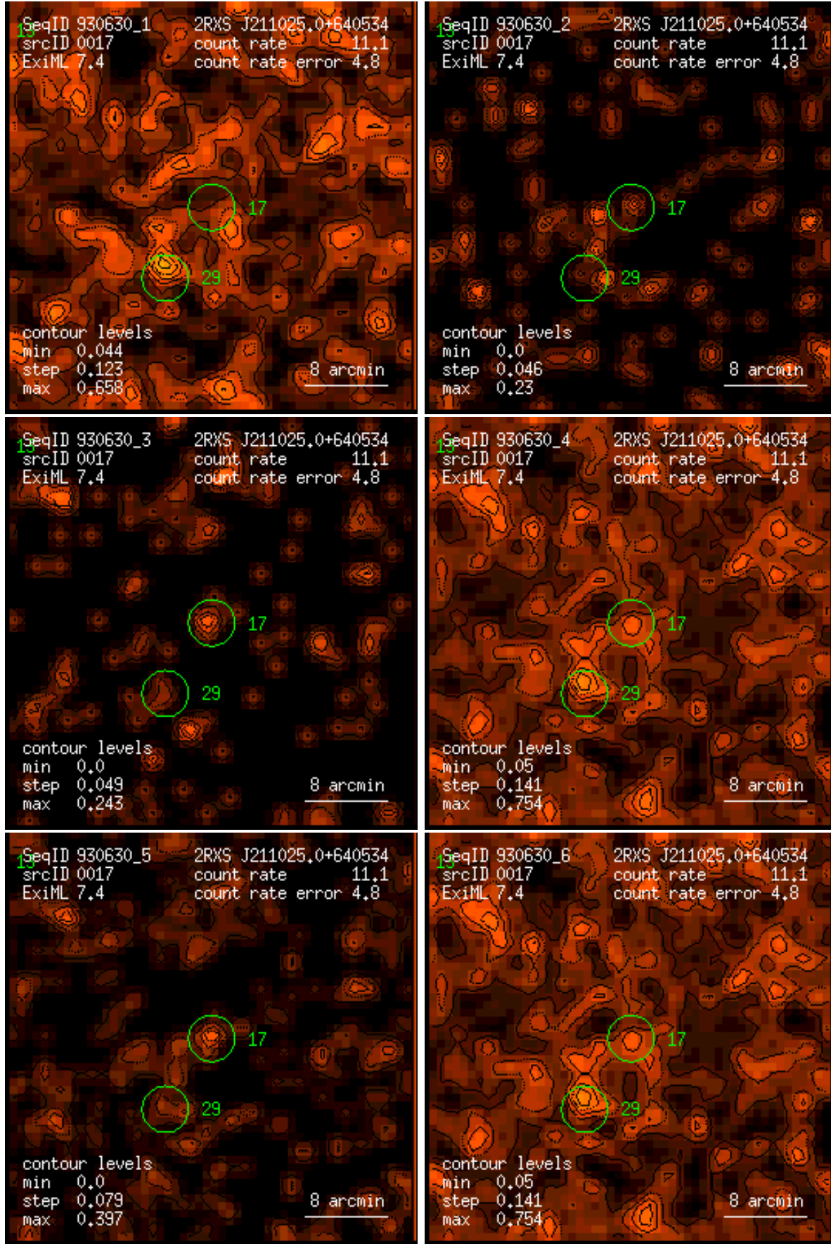
Figure 17: RASS 930630: detection 0017: band rate images, Gaussian filter: (1) PSPC channels 11 – 41, (2) 52 – 90, (3) 91 – 201, (4) 11 – 235, (5) 52 – 201, (6) 11 – 201. Broad band rates in counts/ks. Band rate contour levels in counts/ks/arcmin 2 .
