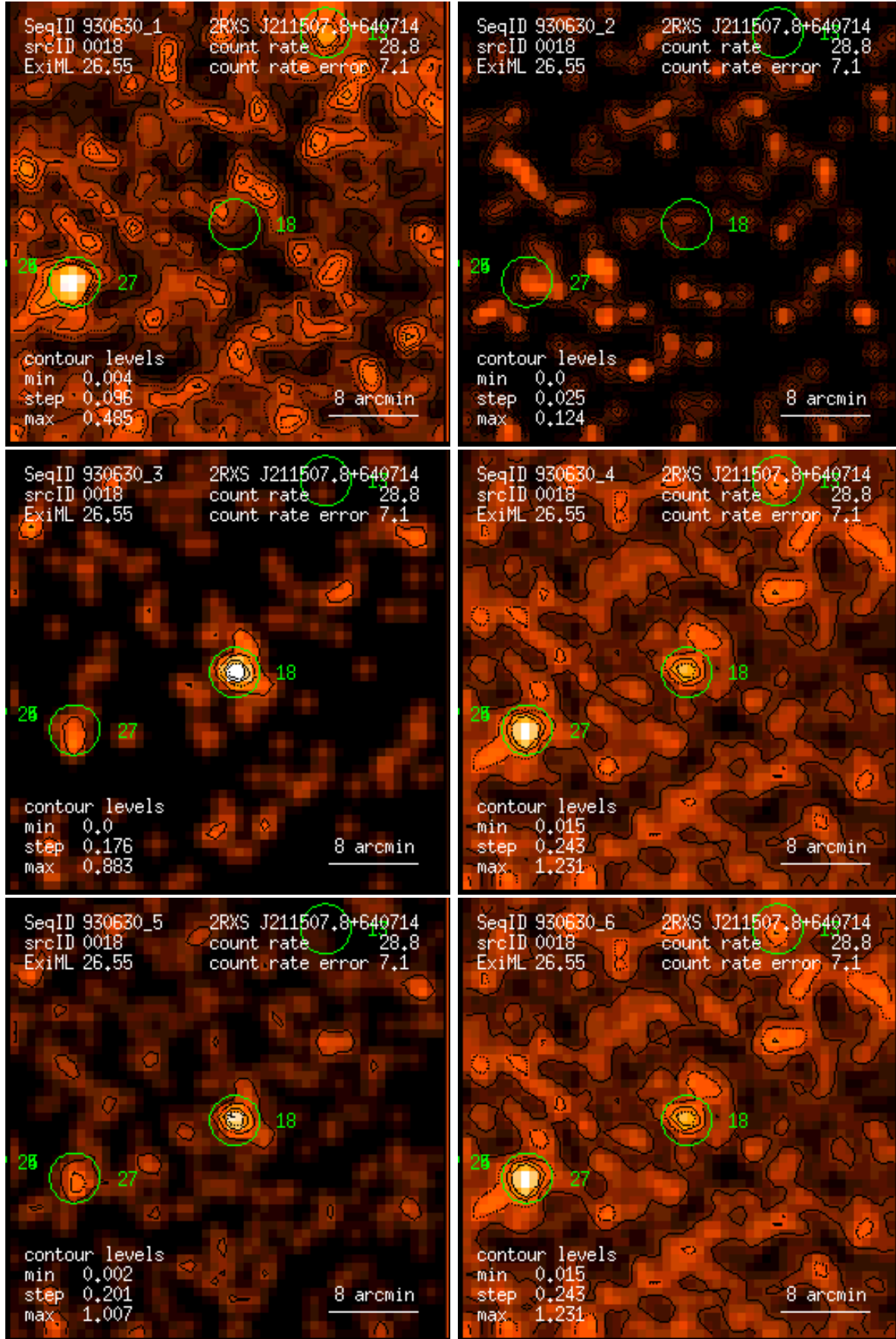
Figure 18: RASS 930630: detection 0018: band rate images, Gaussian filter: (1) PSPC channels 11 – 41, (2) 52 – 90, (3) 91 – 201, (4) 11 – 235, (5) 52 – 201, (6) 11 – 201. Broad band rates in counts/ks. Band rate contour levels in counts/ks/arcmin 2 .
