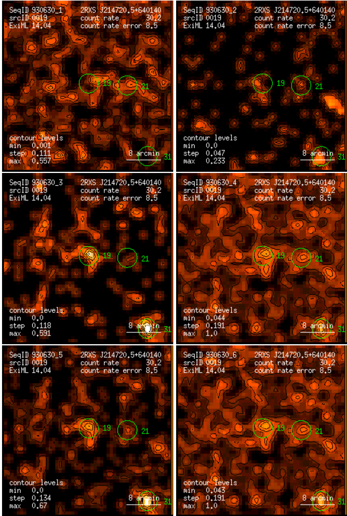
Figure 19: RASS 930630: detection 0019: band rate images, Gaussian filter: (1) PSPC channels 11 – 41, (2) 52 – 90, (3) 91 – 201, (4) 11 – 235, (5) 52 – 201, (6) 11 – 201. Broad band rates in counts/ks. Band rate contour levels in counts/ks/arcmin 2 .
