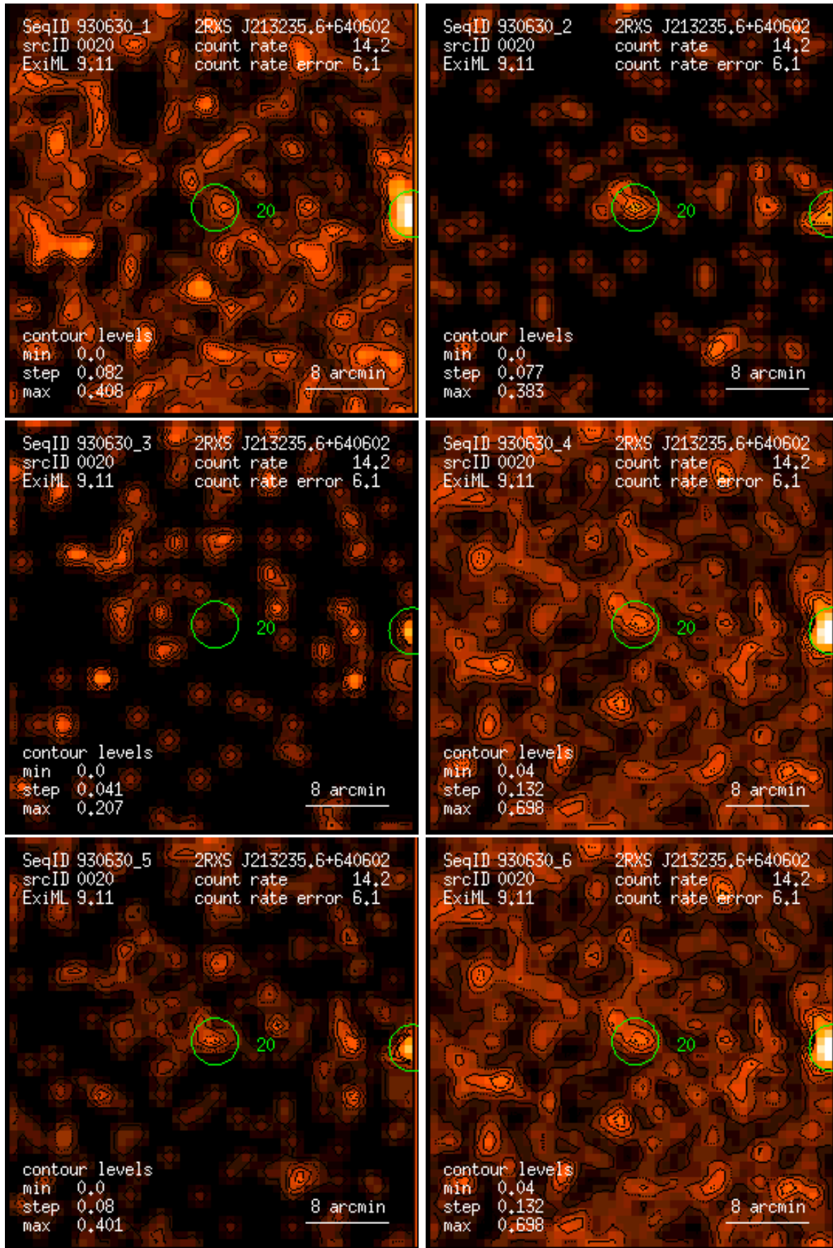
Figure 20: RASS 930630: detection 0020: band rate images, Gaussian filter: (1) PSPC channels 11 – 41, (2) 52 – 90, (3) 91 – 201, (4) 11 – 235, (5) 52 – 201, (6) 11 – 201. Broad band rates in counts/ks. Band rate contour levels in counts/ks/arcmin 2 .
