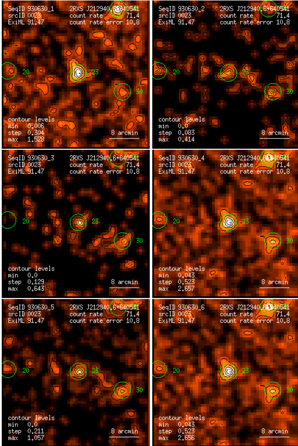
Figure 23: RASS 930630: detection 0023: band rate images, Gaussian filter: (1) PSPC channels 11 – 41, (2) 52 – 90, (3) 91 – 201, (4) 11 – 235, (5) 52 – 201, (6) 11 – 201. Broad band rates in counts/ks. Band rate contour levels in counts/ks/arcmin 2 .
