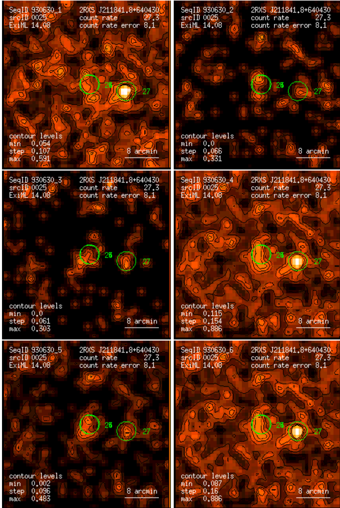
Figure 25: RASS 930630: detection 0025: band rate images, Gaussian filter: (1) PSPC channels 11 – 41, (2) 52 – 90, (3) 91 – 201, (4) 11 – 235, (5) 52 – 201, (6) 11 – 201. Broad band rates in counts/ks. Band rate contour levels in counts/ks/arcmin 2 .
