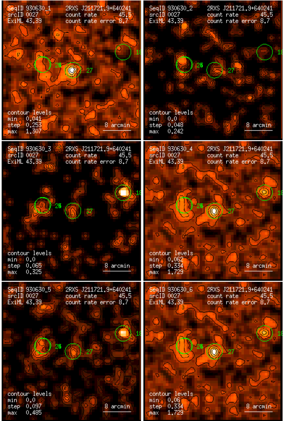
Figure 27: RASS 930630: detection 0027: band rate images, Gaussian filter: (1) PSPC channels 11 – 41, (2) 52 – 90, (3) 91 – 201, (4) 11 – 235, (5) 52 – 201, (6) 11 – 201. Broad band rates in counts/ks. Band rate contour levels in counts/ks/arcmin 2 .
