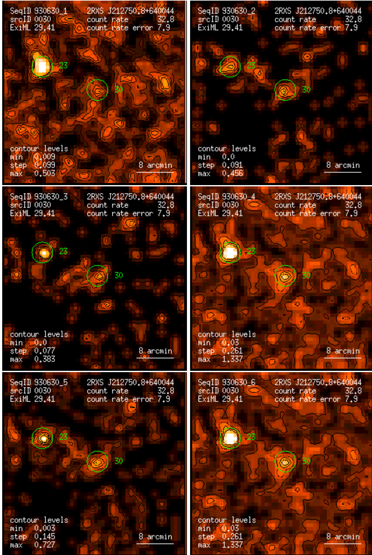
Figure 30: RASS 930630: detection 0030: band rate images, Gaussian filter: (1) PSPC channels 11 – 41, (2) 52 – 90, (3) 91 – 201, (4) 11 – 235, (5) 52 – 201, (6) 11 – 201. Broad band rates in counts/ks. Band rate contour levels in counts/ks/arcmin 2 .
