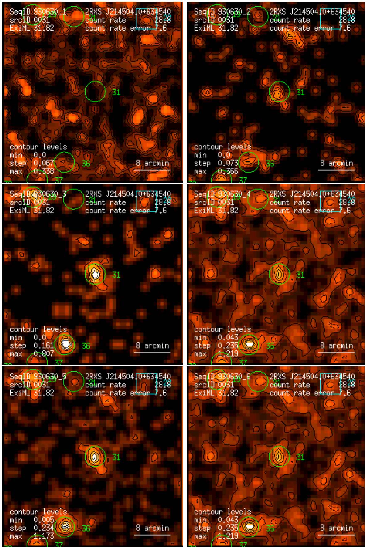
Figure 31: RASS 930630: detection 0031: band rate images, Gaussian filter: (1) PSPC channels 11 – 41, (2) 52 – 90, (3) 91 – 201, (4) 11 – 235, (5) 52 – 201, (6) 11 – 201. Broad band rates in counts/ks. Band rate contour levels in counts/ks/arcmin 2 .
