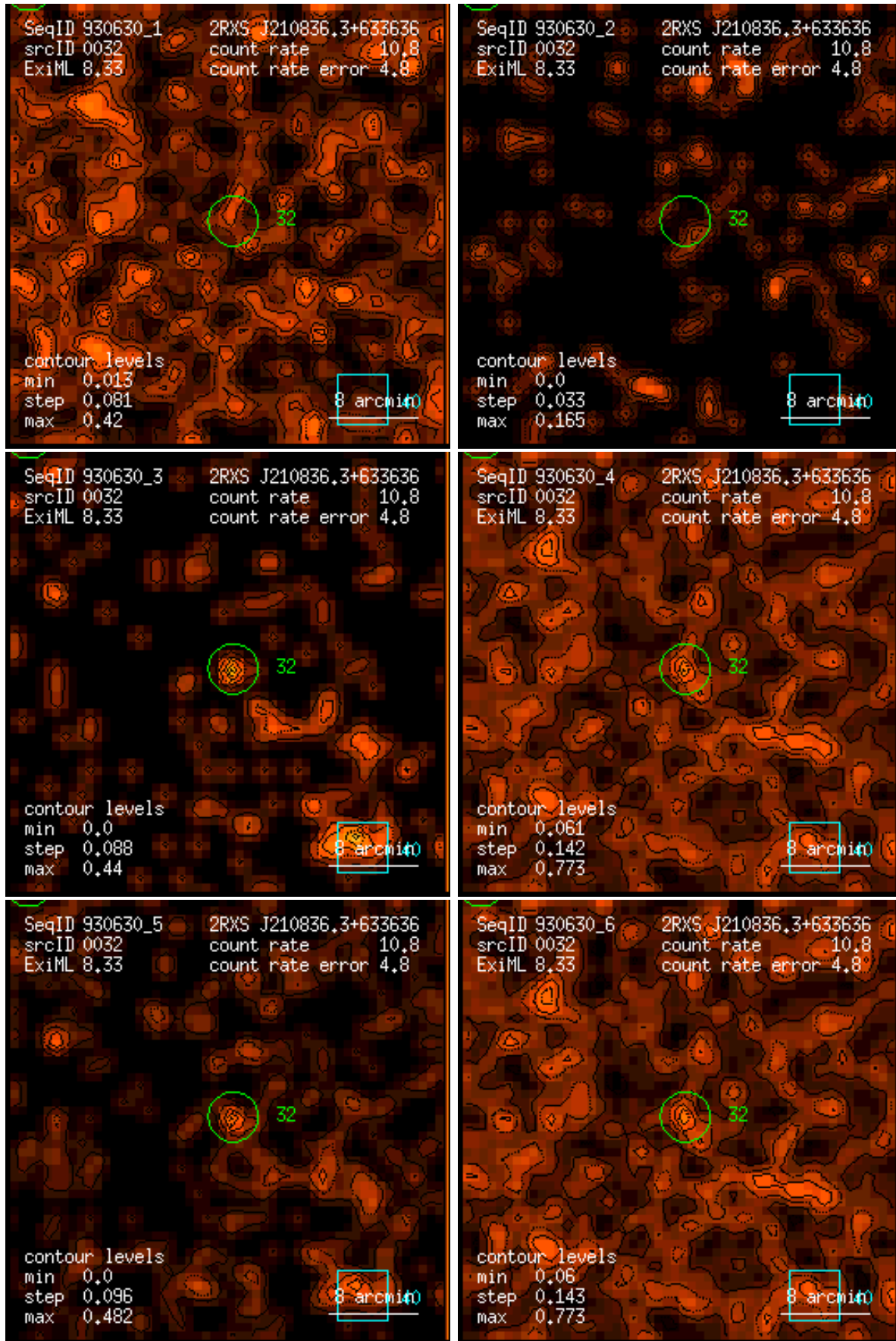
Figure 32: RASS 930630: detection 0032: band rate images, Gaussian filter: (1) PSPC channels 11 – 41, (2) 52 – 90, (3) 91 – 201, (4) 11 – 235, (5) 52 – 201, (6) 11 – 201. Broad band rates in counts/ks. Band rate contour levels in counts/ks/arcmin 2 .
