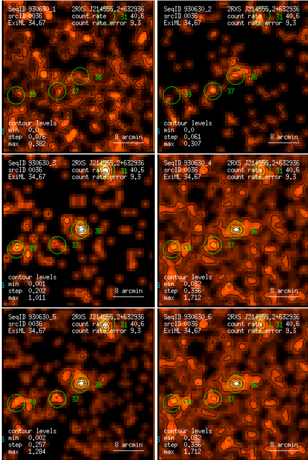
Figure 36: RASS 930630: detection 0036: band rate images, Gaussian filter: (1) PSPC channels 11 – 41, (2) 52 – 90, (3) 91 – 201, (4) 11 – 235, (5) 52 – 201, (6) 11 – 201. Broad band rates in counts/ks. Band rate contour levels in counts/ks/arcmin 2 .
