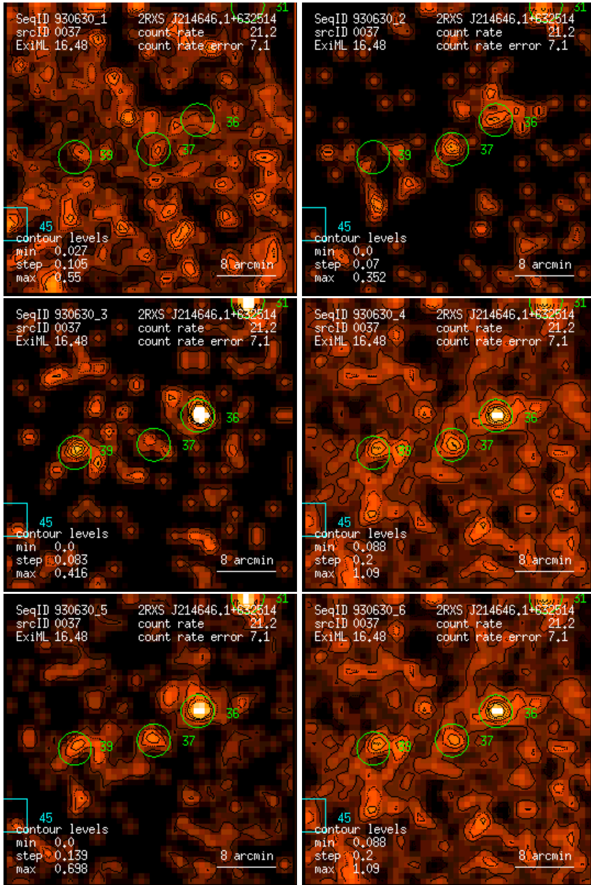
Figure 37: RASS 930630: detection 0037: band rate images, Gaussian filter: (1) PSPC channels 11 – 41, (2) 52 – 90, (3) 91 – 201, (4) 11 – 235, (5) 52 – 201, (6) 11 – 201. Broad band rates in counts/ks. Band rate contour levels in counts/ks/arcmin 2 .
