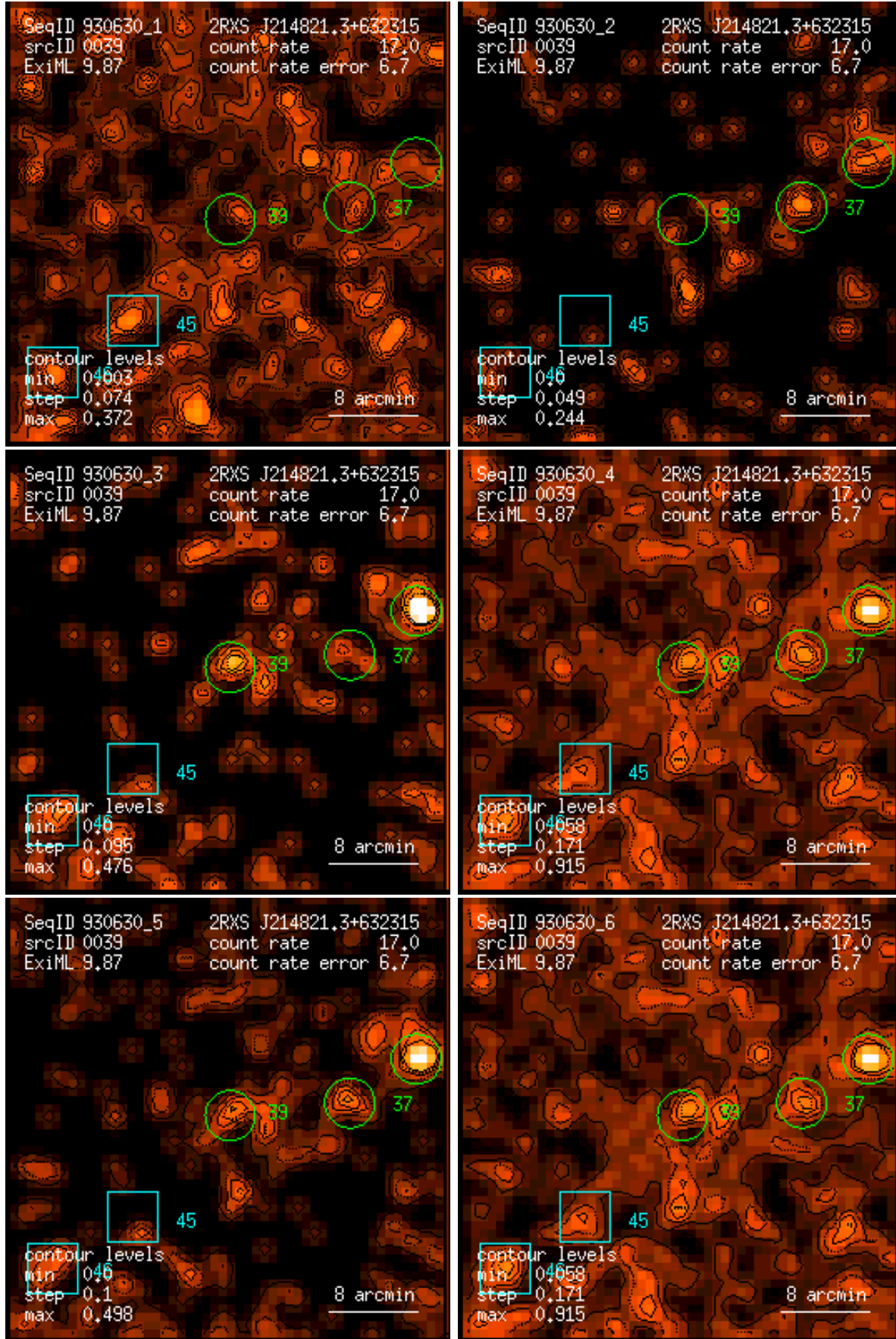
Figure 39: RASS 930630: detection 0039: band rate images, Gaussian filter: (1) PSPC channels 11 – 41, (2) 52 – 90, (3) 91 – 201, (4) 11 – 235, (5) 52 – 201, (6) 11 – 201. Broad band rates in counts/ks. Band rate contour levels in counts/ks/arcmin 2 .
