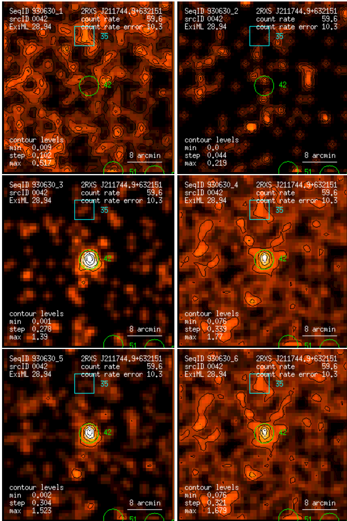
Figure 42: RASS 930630: detection 0042: band rate images, Gaussian filter: (1) PSPC channels 11 – 41, (2) 52 – 90, (3) 91 – 201, (4) 11 – 235, (5) 52 – 201, (6) 11 – 201. Broad band rates in counts/ks. Band rate contour levels in counts/ks/arcmin 2 .
