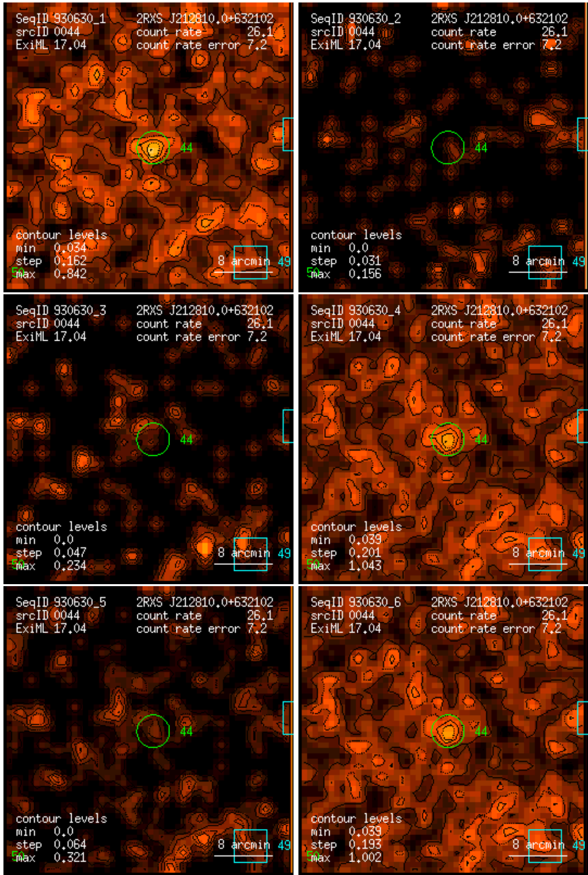
Figure 44: RASS 930630: detection 0044: band rate images, Gaussian filter: (1) PSPC channels 11 – 41, (2) 52 – 90, (3) 91 – 201, (4) 11 – 235, (5) 52 – 201, (6) 11 – 201. Broad band rates in counts/ks. Band rate contour levels in counts/ks/arcmin 2 .
