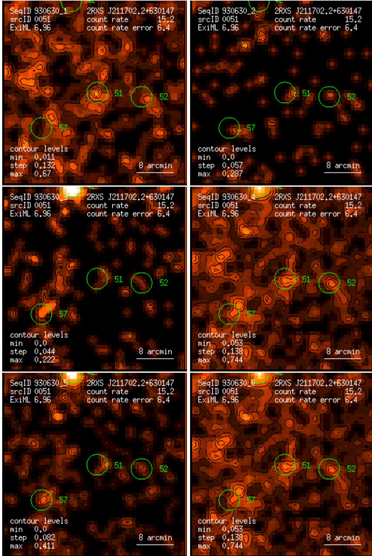
Figure 51: RASS 930630: detection 0051: band rate images, Gaussian filter: (1) PSPC channels 11 – 41, (2) 52 – 90, (3) 91 – 201, (4) 11 – 235, (5) 52 – 201, (6) 11 – 201. Broad band rates in counts/ks. Band rate contour levels in counts/ks/arcmin 2 .
