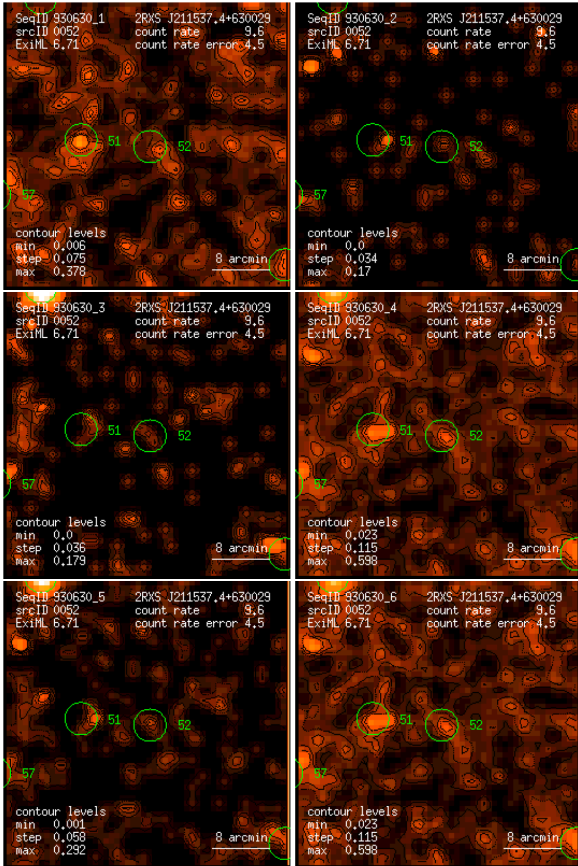
Figure 52: RASS 930630: detection 0052: band rate images, Gaussian filter: (1) PSPC channels 11 – 41, (2) 52 – 90, (3) 91 – 201, (4) 11 – 235, (5) 52 – 201, (6) 11 – 201. Broad band rates in counts/ks. Band rate contour levels in counts/ks/arcmin 2 .
