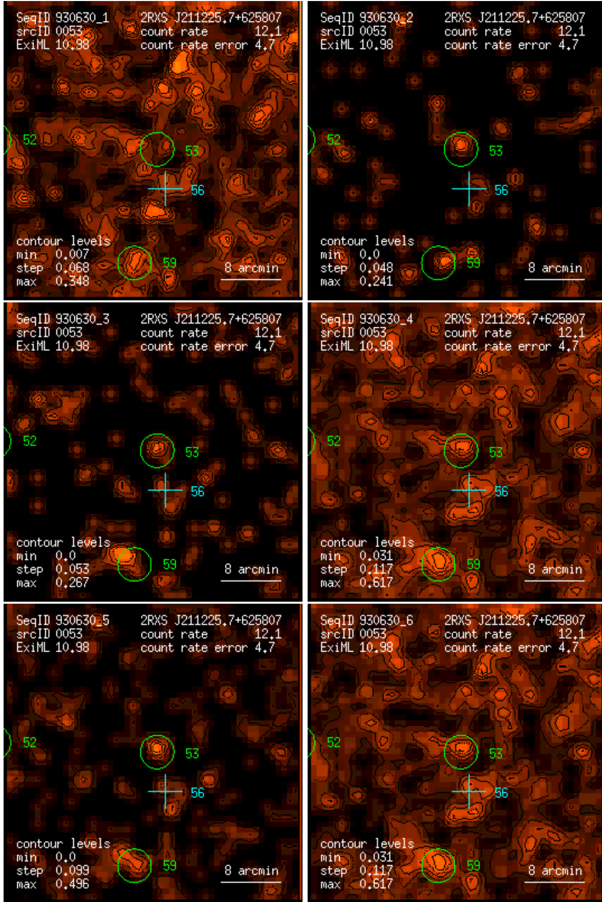
Figure 53: RASS 930630: detection 0053: band rate images, Gaussian filter: (1) PSPC channels 11 – 41, (2) 52 – 90, (3) 91 – 201, (4) 11 – 235, (5) 52 – 201, (6) 11 – 201. Broad band rates in counts/ks. Band rate contour levels in counts/ks/arcmin 2 .
