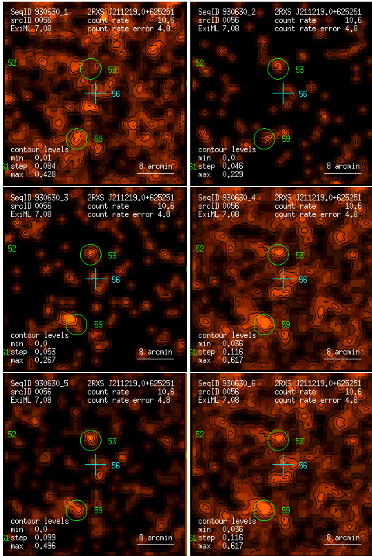
Figure 56: RASS 930630: detection 0056: band rate images, Gaussian filter: (1) PSPC channels 11 – 41, (2) 52 – 90, (3) 91 – 201, (4) 11 – 235, (5) 52 – 201, (6) 11 – 201. Broad band rates in counts/ks. Band rate contour levels in counts/ks/arcmin 2 .
