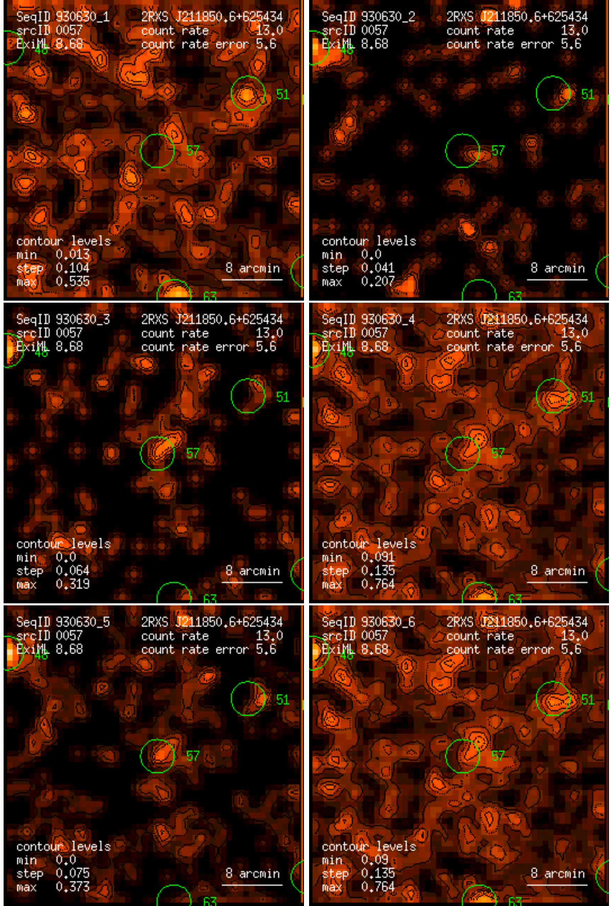
Figure 57: RASS 930630: detection 0057: band rate images, Gaussian filter: (1) PSPC channels 11 – 41, (2) 52 – 90, (3) 91 – 201, (4) 11 – 235, (5) 52 – 201, (6) 11 – 201. Broad band rates in counts/ks. Band rate contour levels in counts/ks/arcmin 2 .
