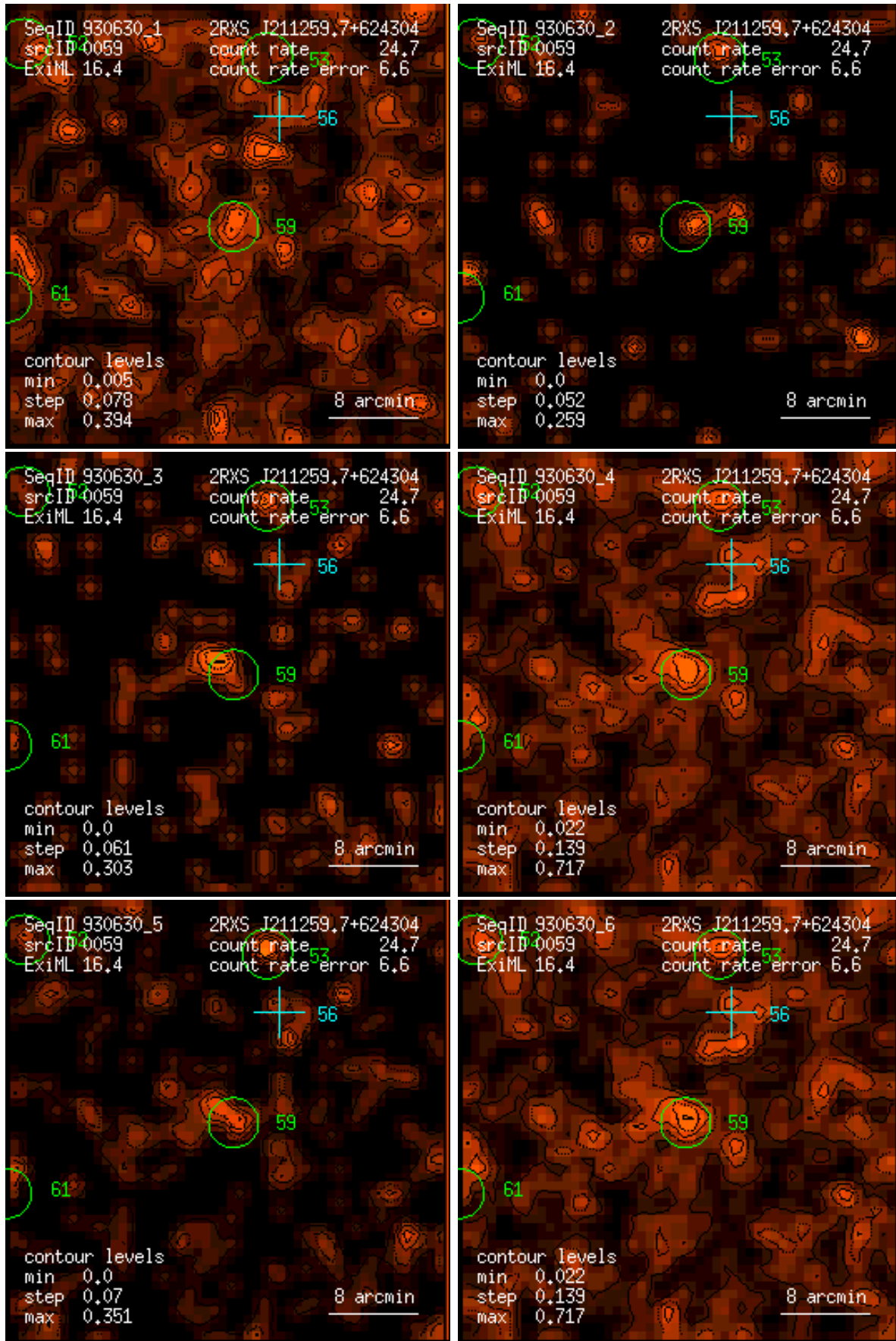
Figure 59: RASS 930630: detection 0059: band rate images, Gaussian filter: (1) PSPC channels 11 – 41, (2) 52 – 90, (3) 91 – 201, (4) 11 – 235, (5) 52 – 201, (6) 11 – 201. Broad band rates in counts/ks. Band rate contour levels in counts/ks/arcmin 2 .
