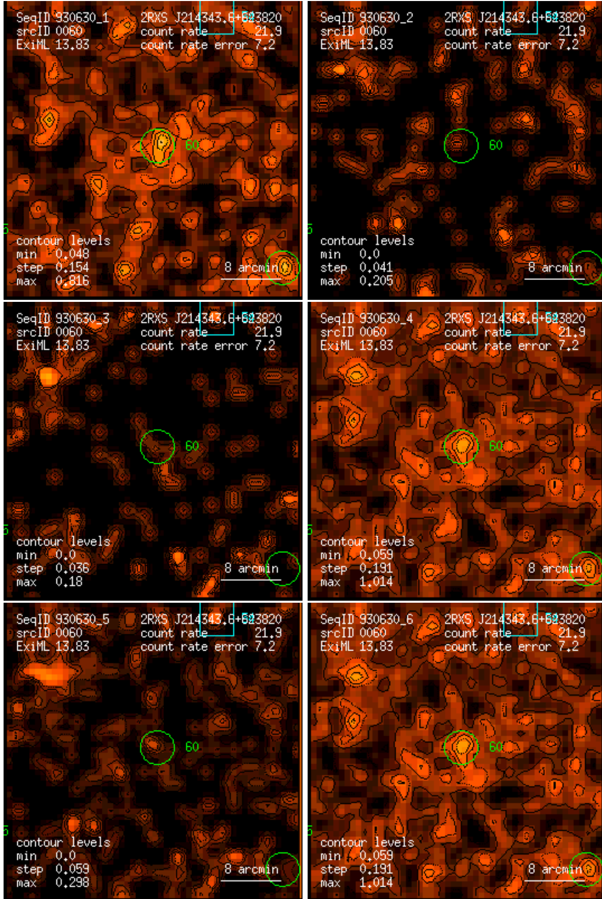
Figure 60: RASS 930630: detection 0060: band rate images, Gaussian filter: (1) PSPC channels 11 – 41, (2) 52 – 90, (3) 91 – 201, (4) 11 – 235, (5) 52 – 201, (6) 11 – 201. Broad band rates in counts/ks. Band rate contour levels in counts/ks/arcmin 2 .
