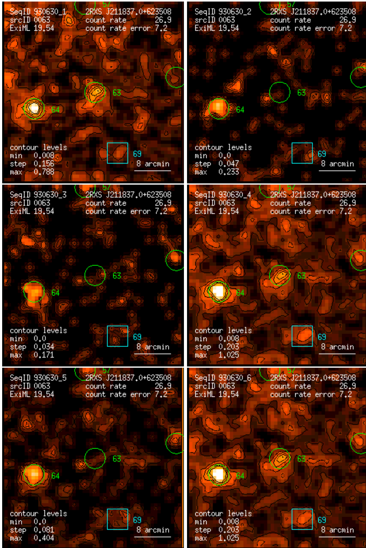
Figure 63: RASS 930630: detection 0063: band rate images, Gaussian filter: (1) PSPC channels 11 – 41, (2) 52 – 90, (3) 91 – 201, (4) 11 – 235, (5) 52 – 201, (6) 11 – 201. Broad band rates in counts/ks. Band rate contour levels in counts/ks/arcmin 2 .
